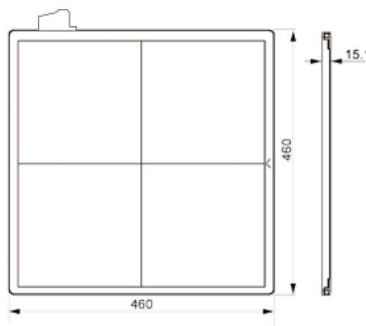
MARS1717V(Wired Version)
